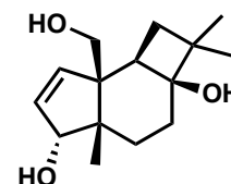
(-)-Punctatin A
