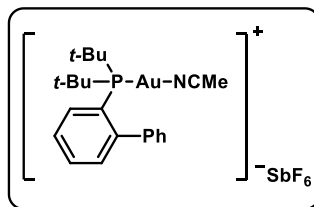
Echavarren's catalyst
