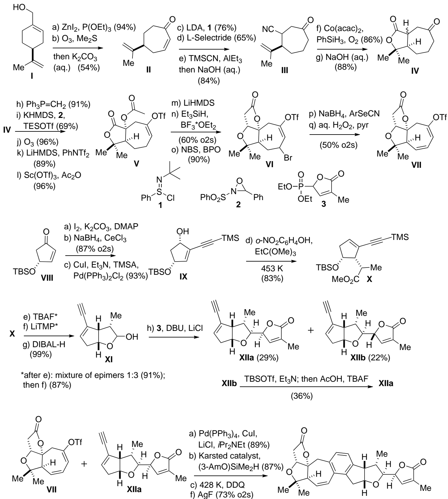
Schisandraceae bisnortriterpenoid Rubriflordilactone B
