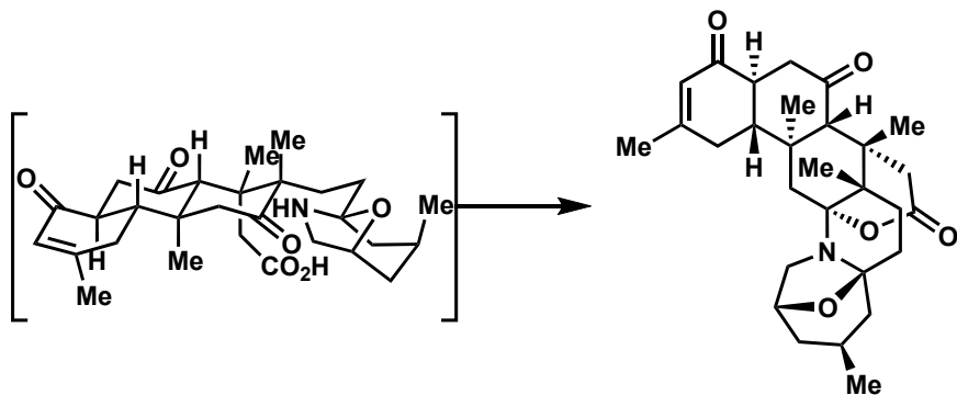
Norzoanthamine
