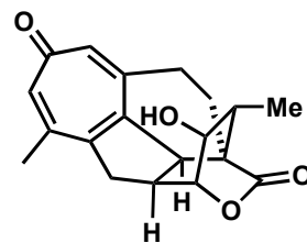
hainanolidol
