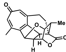
harringtonolide
