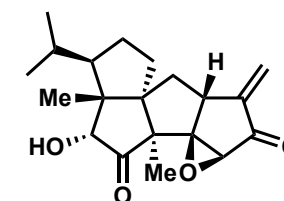
(-)-Crinipellin A
