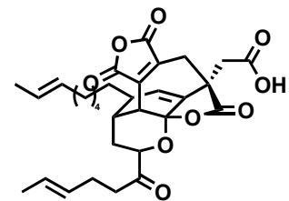
(±)-Phomoidride D
