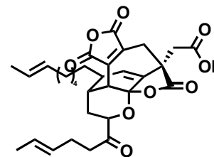
(±)-Phomoidride D
